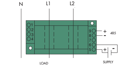
CRD4150 Dual Element, 3-Wire
