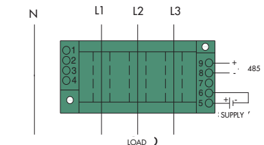
CRD4170 3 Element, 4-Wire
