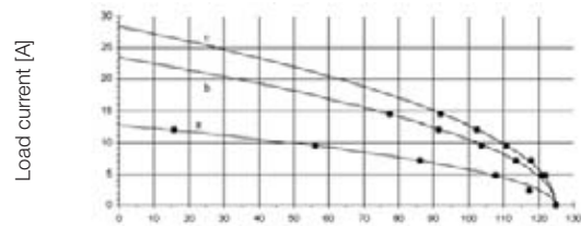
HEE 10-pole Ambient temperature [°C]
