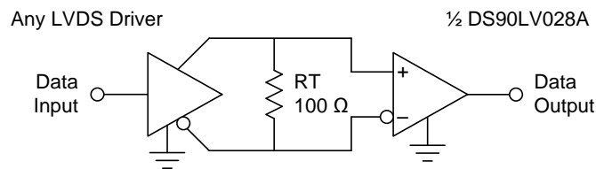
Figure 20. Point-to-Point Application
