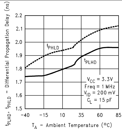
Figure 8. Differential Propagation Delay vs Ambient Temperature
