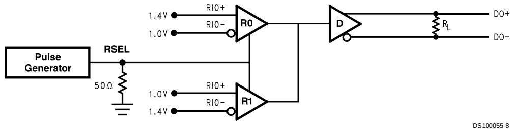
FIGURE 6. Receiver Select to Driver Propagation Delay Test Circuit
