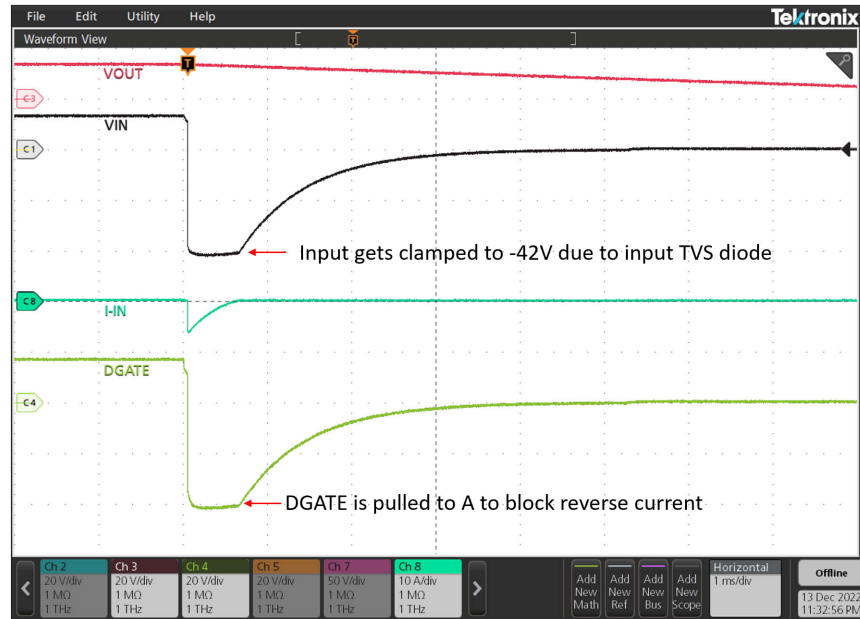
Figure 10-2. ISO 7637-2 Pulse 1
