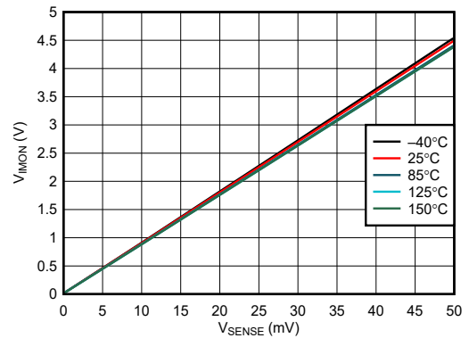
Figure 7-22. Current Monitor Output vs Sense Voltage ( R_{IMON} = 5k\Omega , R_{SET} = 50\Omega )
