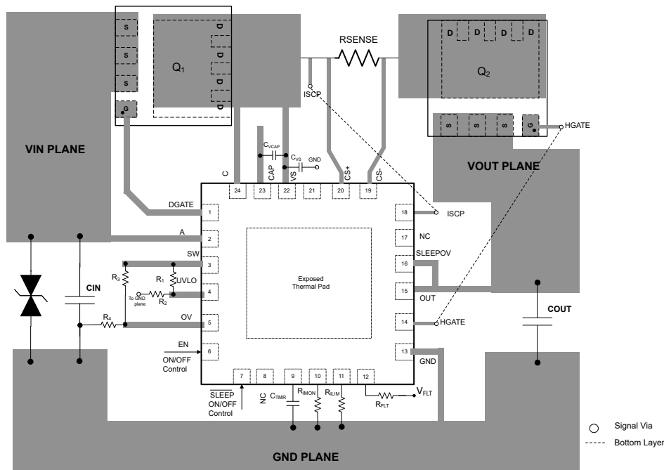
Figure 10-24. Example Layout
