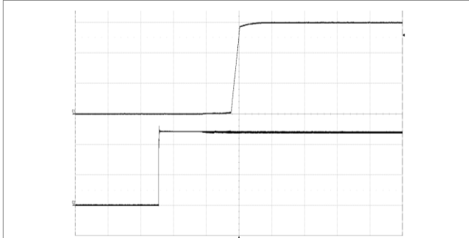
Start-up enabled by connecting V_i at: T_{P1} = +25^{\circ}\text{C} , V_i = 24\text{ V} , I_o = 1\text{ A} electronic load. Top trace: output voltage (5 V/div.). Bottom trace: input voltage (10 V/div.). Time scale: (2 ms/div.).
