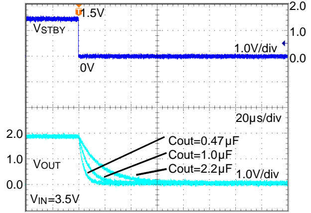
Figure 23. Discharge Time (ROUT=9Ω)
