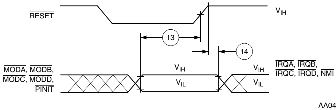
Figure 3-7 Operating Mode Select Timing
