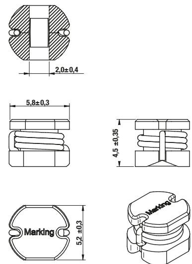
Dimensions (in mm): Size 5848
