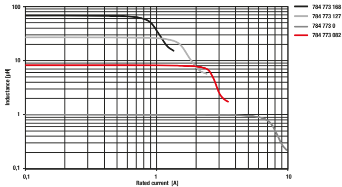
Electrical properties: Size 5848
