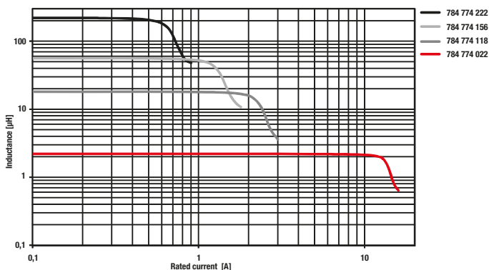
Inductance vs. rated current: Size 5848
