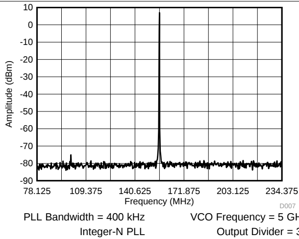
Figure 7. 156.25 ± 78.125-MHz LVPECL Differential Output Spectrum
