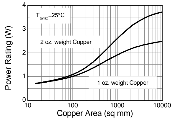
Power Rating vs. Cu Area
