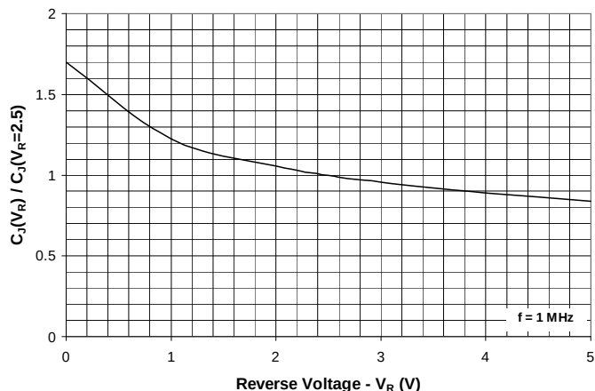
Capacitance vs. Reverse Voltage (Normalized to 2.5 volts)
