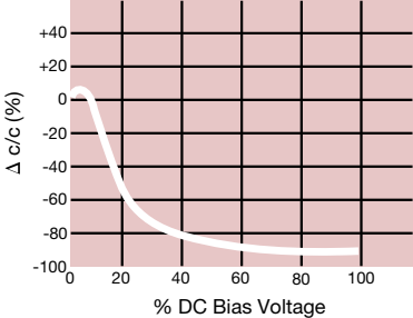
Capacitance Change vs. DC Bias Voltage
