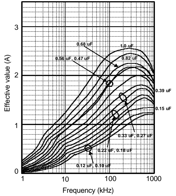
Permissible current
