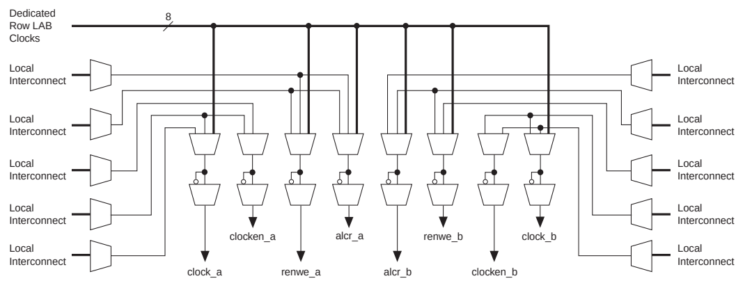
Figure 2-18. M4K RAM Block LAB Row Interface
