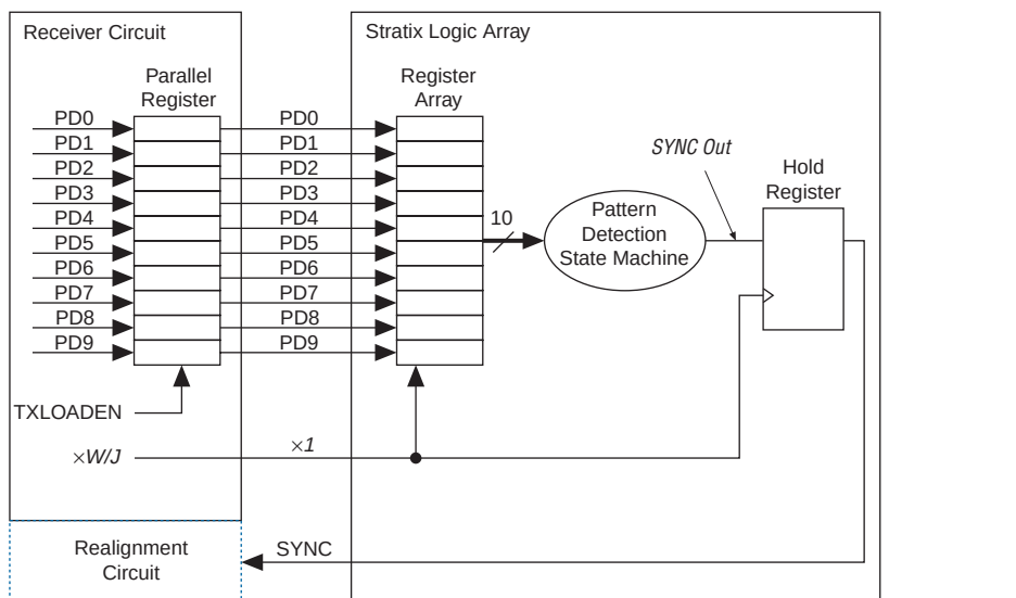
Figure 5–22. SYNC Signal Path to Realignment Circuit
