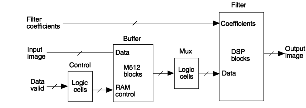
Figure 19–28. Block Diagram on Implementation of 3 \times 3 Convolutional Filter for an 8 \times 8 Pixel Input Image
