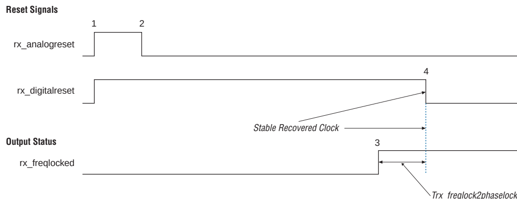
Figure 9–12. Receiver Reset Sequence Waveform
