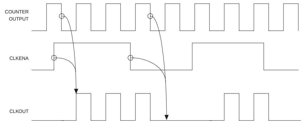
Figure 13–7. extclkena Signals
