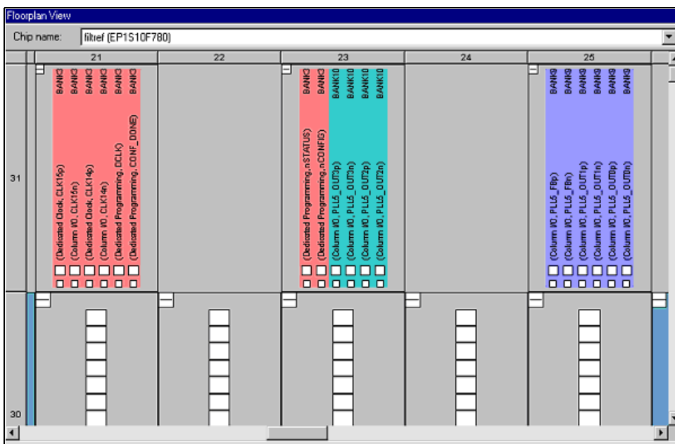
Figure 16–24. Floorplan View Window
