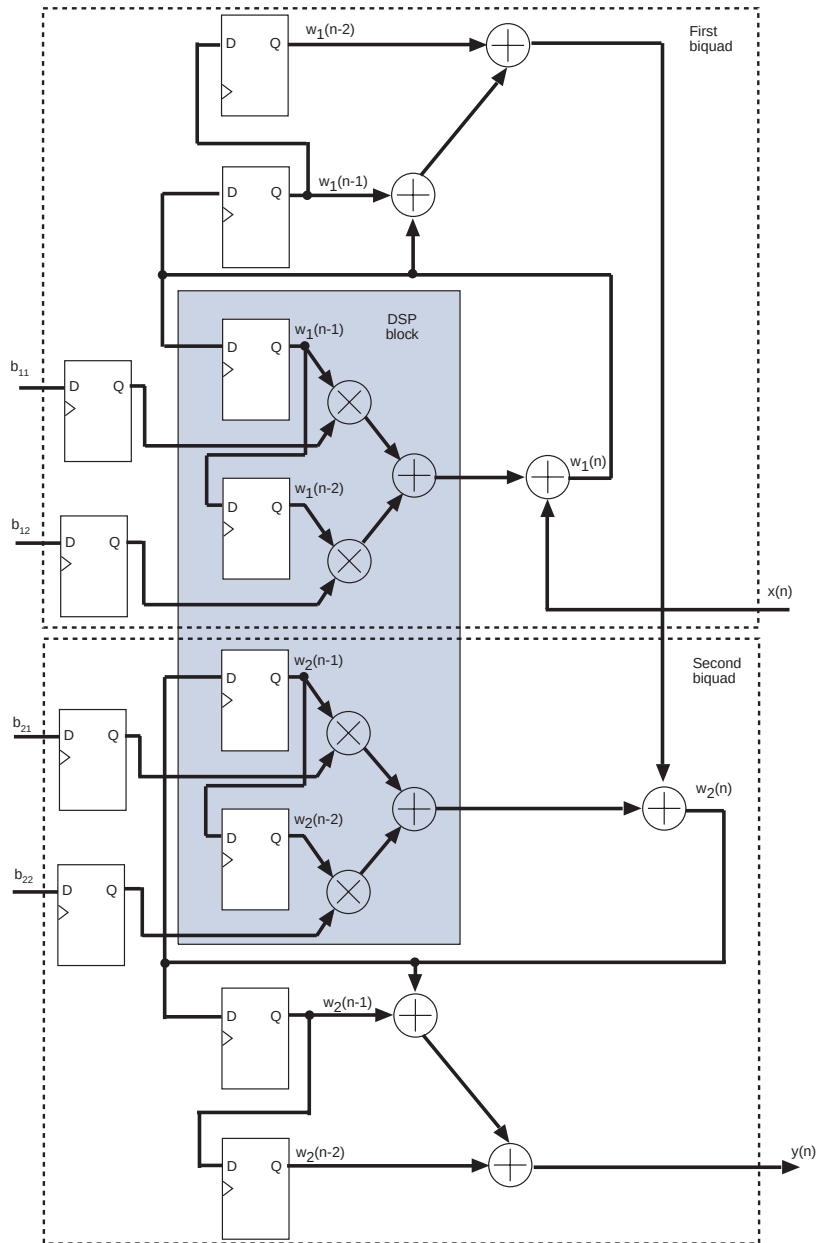
Figure 19–25. Cascaded Butterworth Biquads Note (1)
