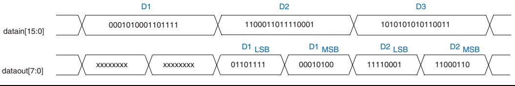
Figure 5–16. Transmitter Byte Serializer in 16- to 8-Bit Mode
