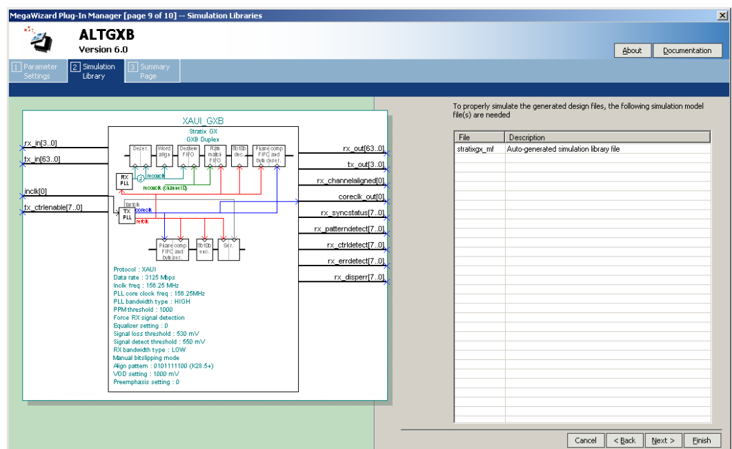
Figure 5–34. MegaWizard Plug-In Manager - altqxb (Page 9)
