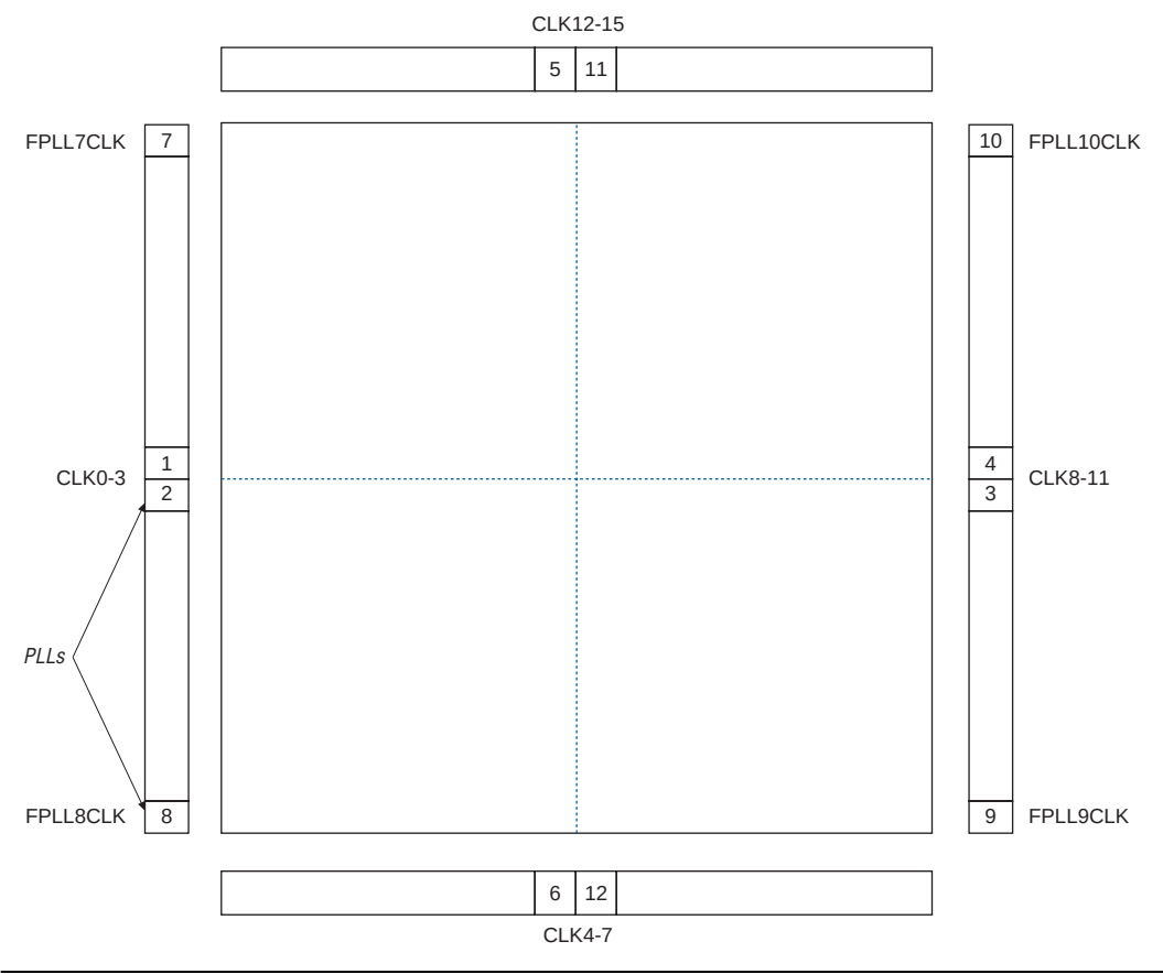
Figure 13–1. Stratix PLL Locations
