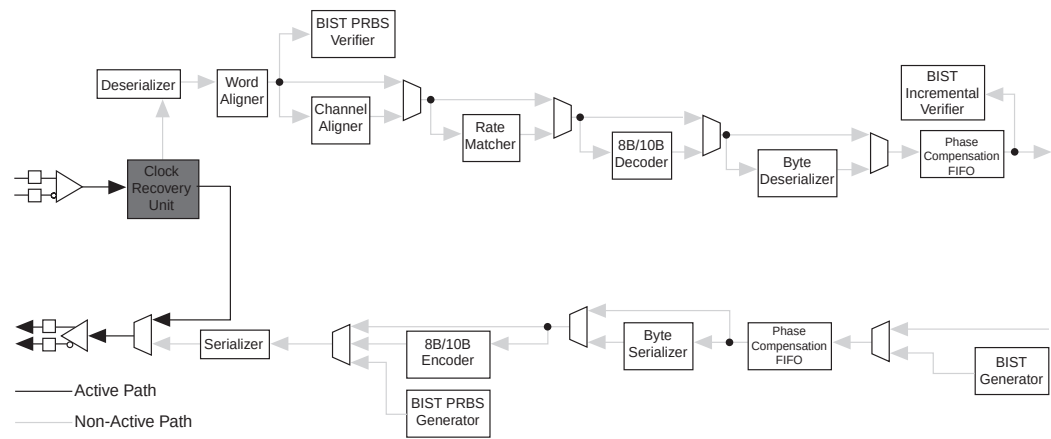
Figure 7–3. Stratix GX Block in Reverse Serial Loopback Mode
