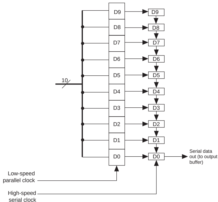
Figure 2–5. Serializer
