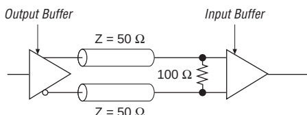
Figure 16–14. LVPECL DC Coupled Termination
