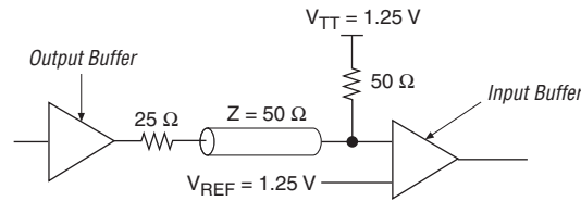
Figure 4-1. 2.5-V SSTL Class I Termination
