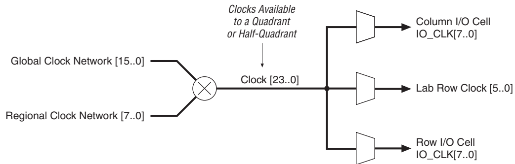
Figure 1–41. Hierarchical Clock Networks Per Quadrant
