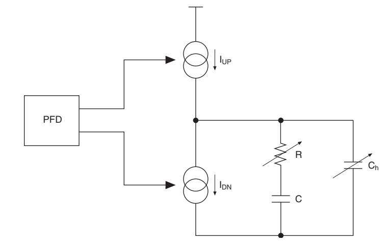
Figure 1–31. Loop Filter Programmable Components
