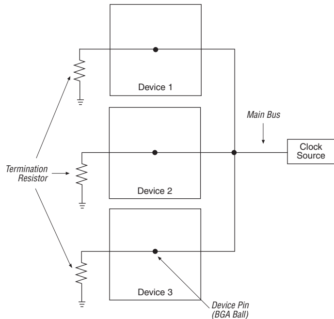
Figure 11–19. Star Routing
