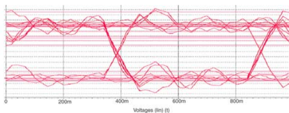
Figure 11-15. Stub Length = 0.5 Inch
