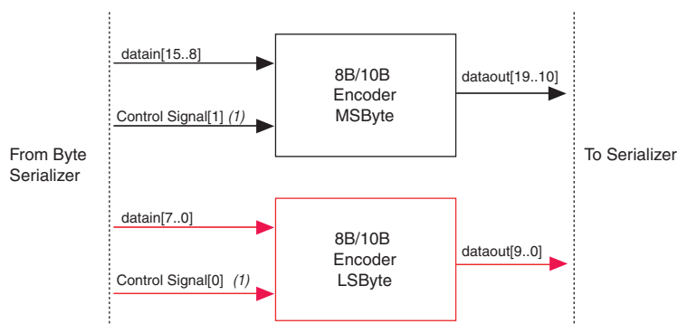
Figure 2–26. 8B/10B Encoder, Single-Width Mode
