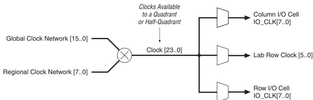
Figure 7–41. Hierarchical Clock Networks Per Quadrant
