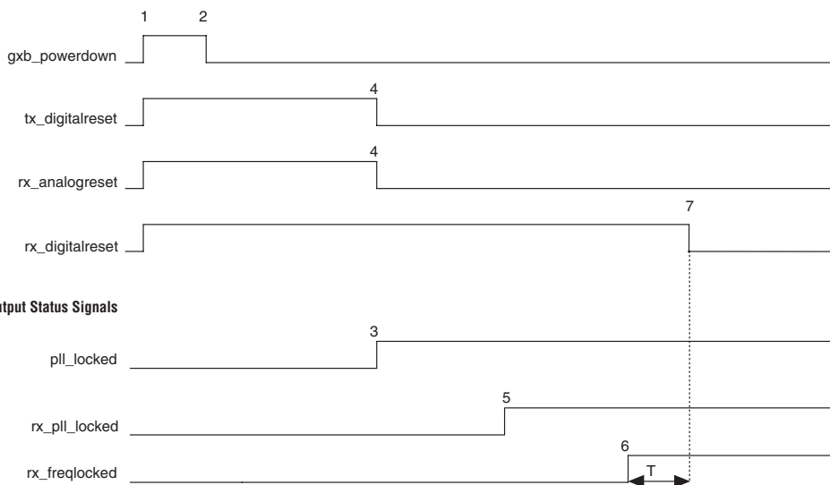
Figure 2–160. Reset Power Signal Timing Waveform
