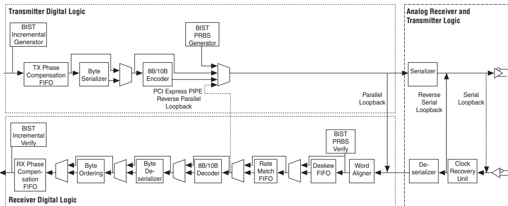
Figure 1–4. Loopback Modes
