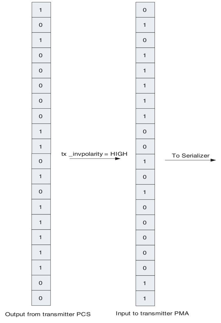
Figure 2–37. Transmitter Polarity Inversion in Double-Width Mode
