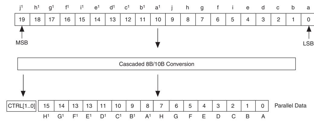
Figure 2–86. 20-Bit to 16-Bit Conversion
