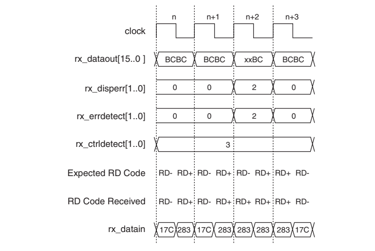
Figure 2–87. Disparity Error
