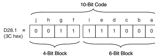
Figure 6-3. Running Disparity Between Sub-Blocks
