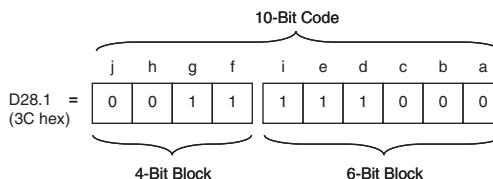
Figure 6-2. 10-Bit Grouping of 6-bit and 4-Bit Sub-Blocks
