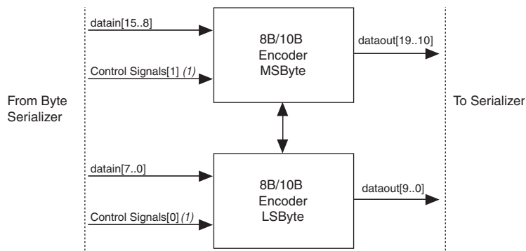
Figure 2–25. 8B/10B Encoder
