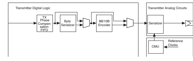
Figure 1–2. Stratix II GX Transmitter Block Diagram
