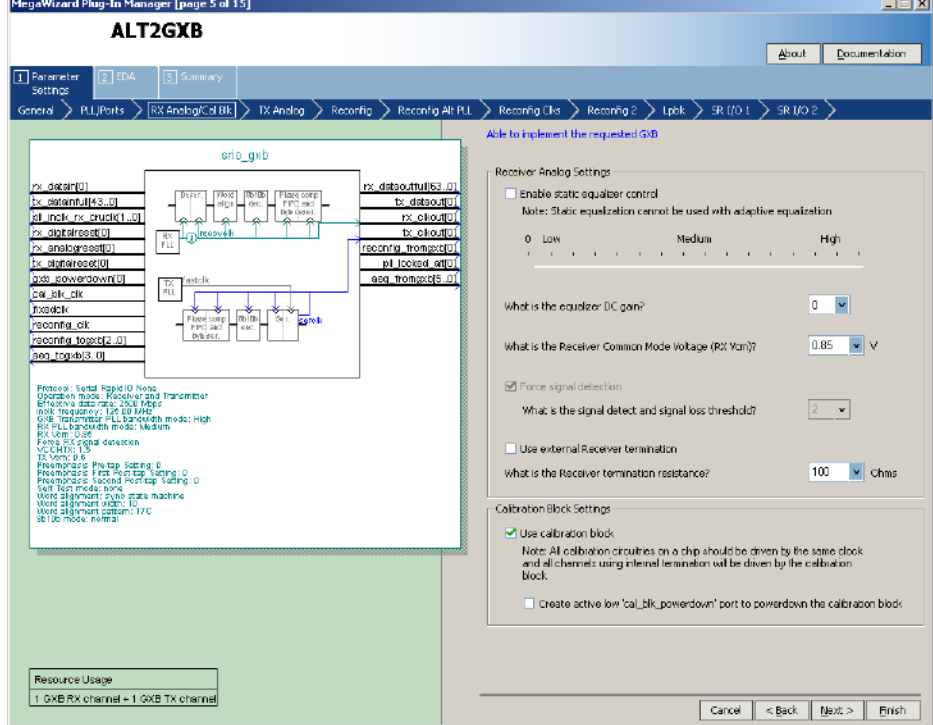
MegaWizard Plug-In Manager [page 5 of 15]
