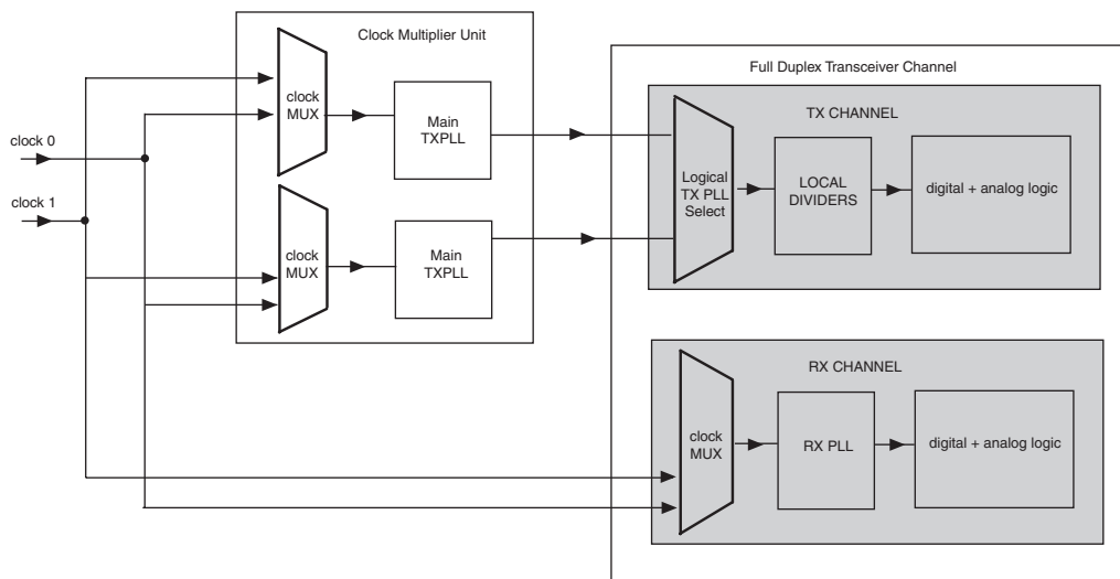
Figure 3–38. Reconfigured Functional Blocks with Channel Reconfiguration Note (1)
