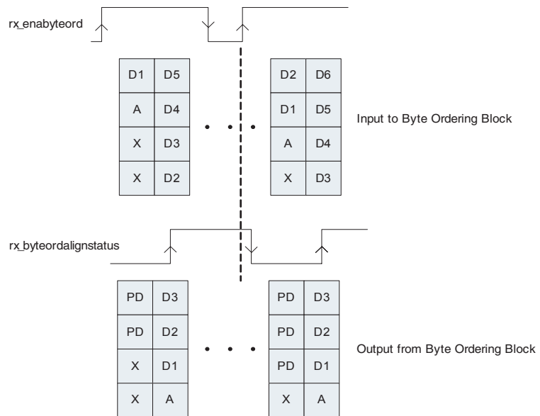
Figure 2–95. User-Controlled Byte Ordering in Double-Width Mode
