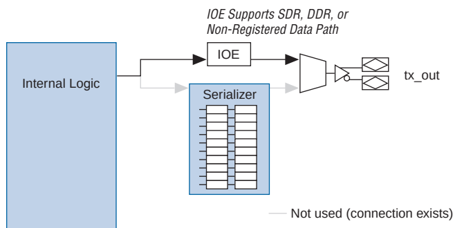
Figure 11–5. Serializer Bypass
