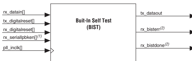
Figure 2–157. Built-In Self Test Mode
