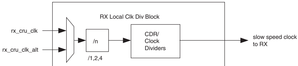
Figure 3–16. Receive Local Clock Divider Block
