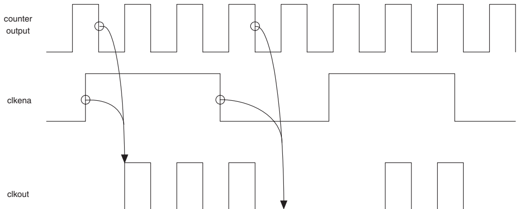
Figure 7–56. Clkena Signals
