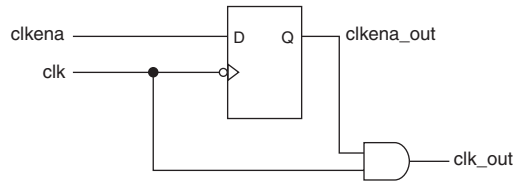
Figure 7–55. clkena Implementation
