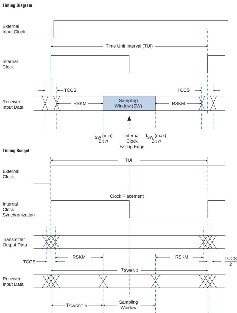
Figure 11–19. Differential High-Speed Timing Diagram and Timing Budget for Non-DPA
