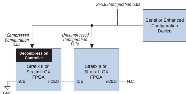
Figure 13–2. Compressed and Uncompressed Configuration Data in the Same Configuration File
