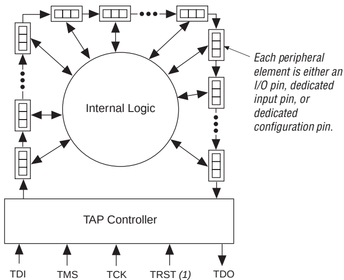
Figure 15–3. Boundary-Scan Register
