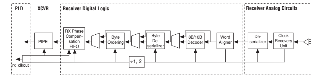
Figure 2–18. Individual Channel Receiver Logic Clocking Without Rate Matching
