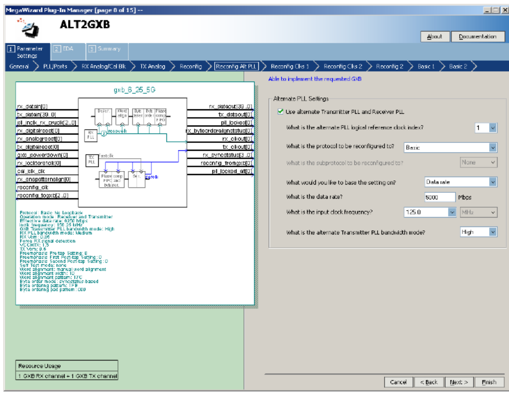
Figure 3–59. Reconfig Alt PLL Tab
