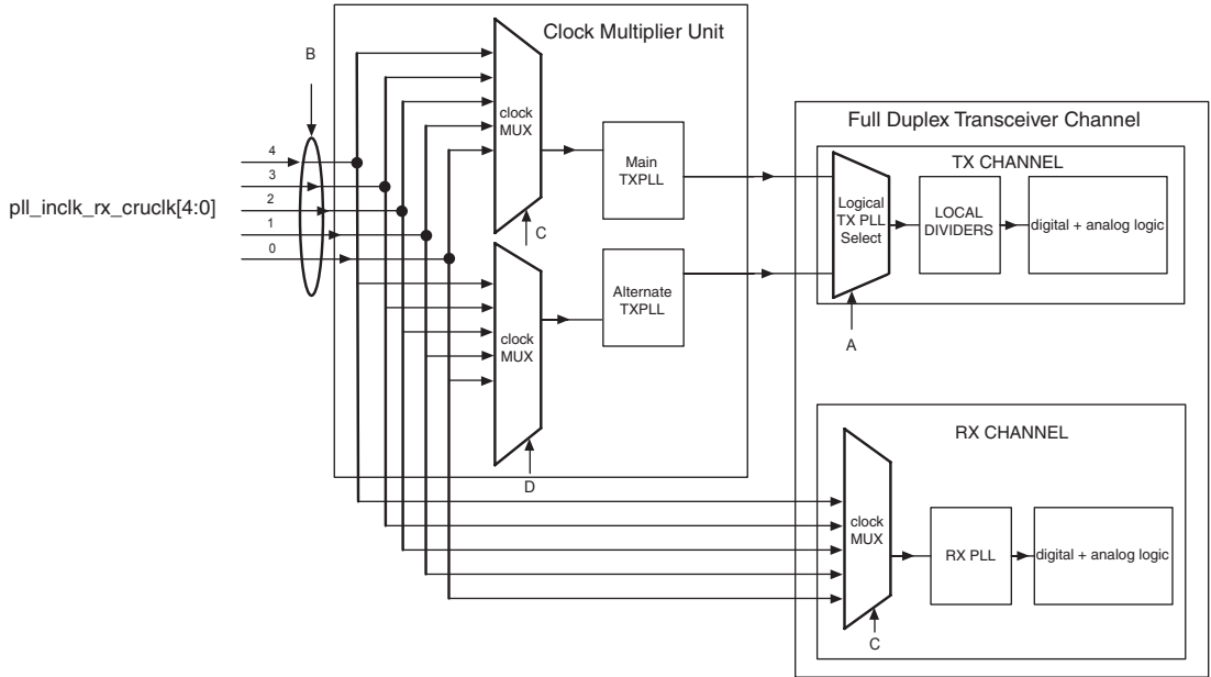
Figure 3–61. Mapping Between the MegaWizard Settings and Hardware Settings
