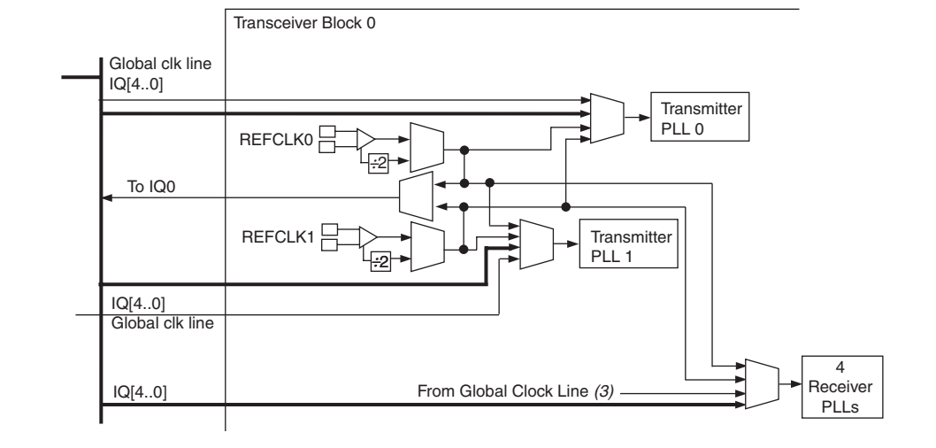
Figure 3–39. Transceiver Block with Global Clock Line Connections
