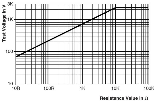
1.2 / 50 Pulse
