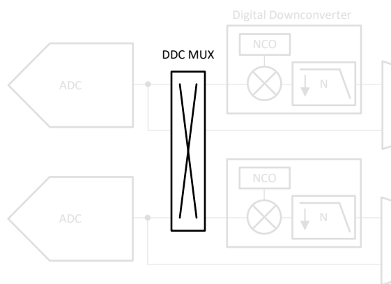
Figure 8-22. DDC MUX
