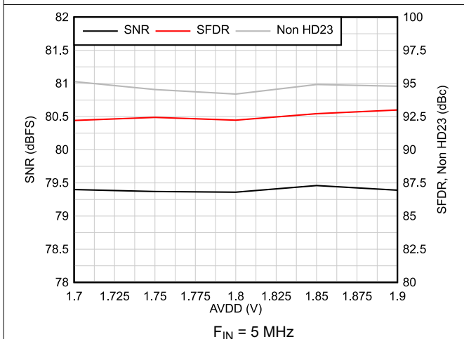
Figure 6-53. AC Performance vs AVDD F_{IN} = 5 \text{ MHz}
