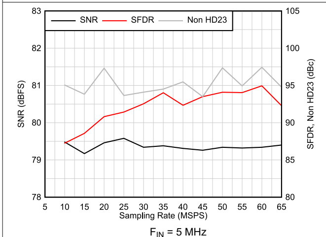
Figure 6-51. AC Performance vs Sampling Rate F_{IN} = 5 \text{ MHz}
