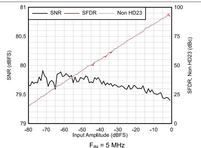
Figure 6-50. AC Performance vs Input Amplitude F_{IN} = 5 \text{ MHz}
