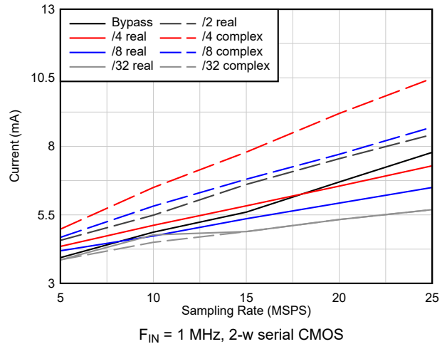
Figure 6-16. I_{OVDD} Current vs Decimation
