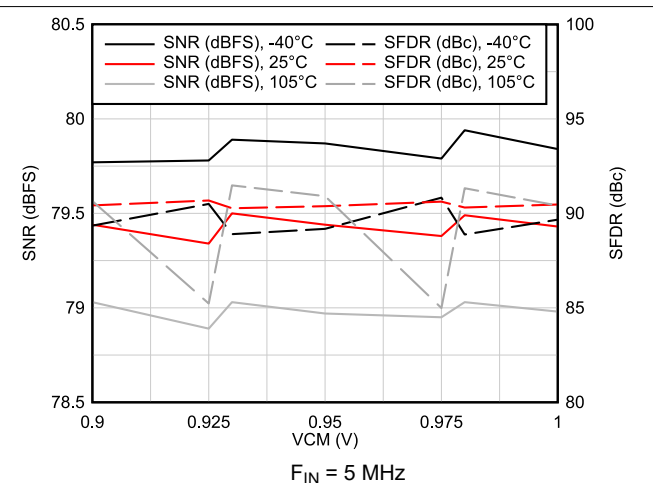
Figure 6-54. AC Performance vs VCM vs Temperature F_{IN} = 5 \text{ MHz}
