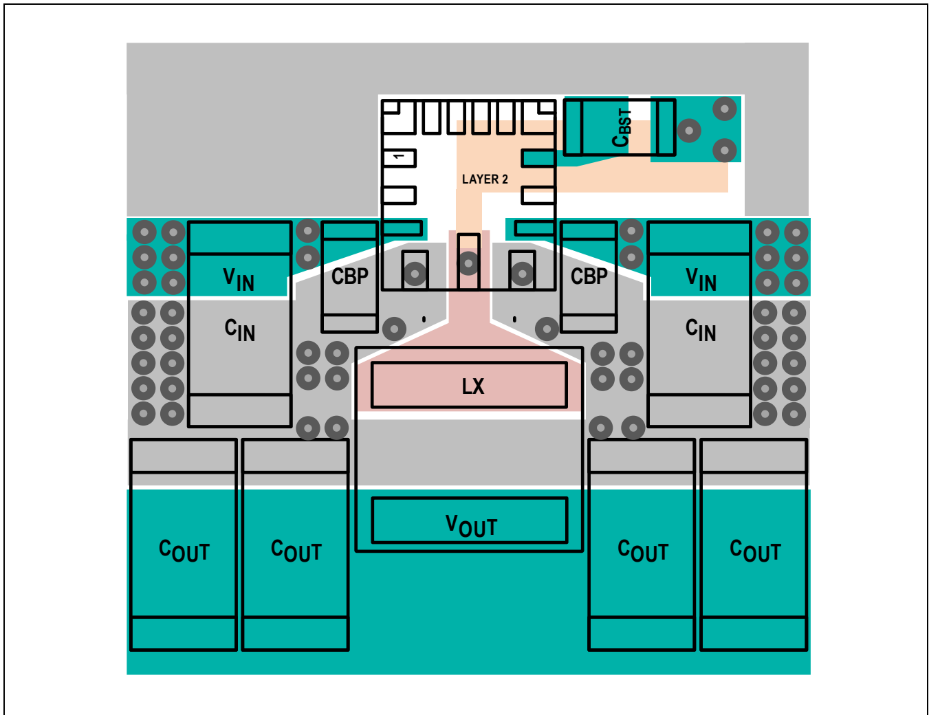
Figure 1. PCB Layout Example
