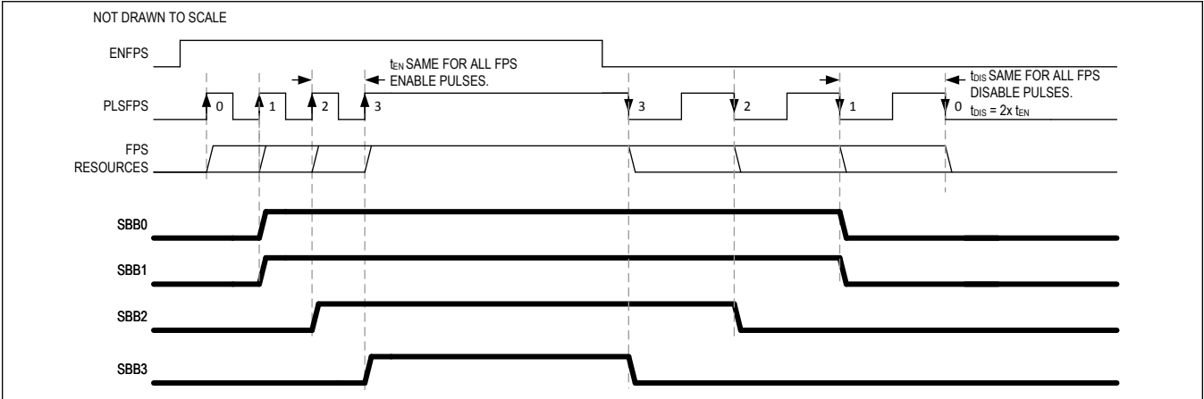
Figure 7. Flexible Power Sequencer Basic Timing Diagram
