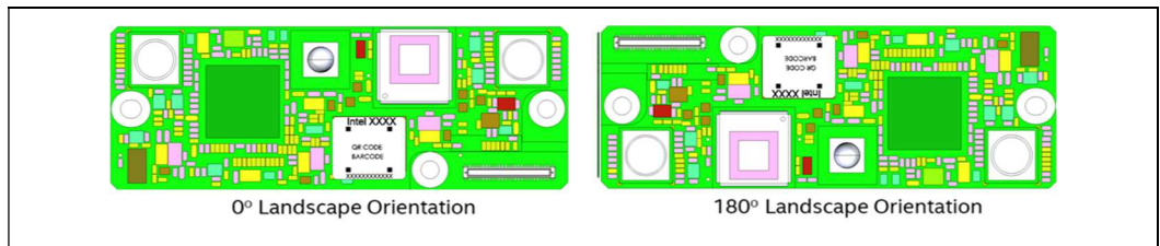
Figure 3-4: Mount Orientation
