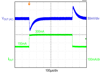
CONDITIONS: 3.3V OUTPUT, PWM MODE
