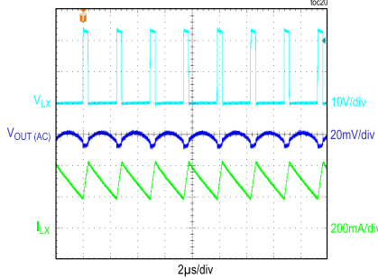
CONDITIONS: 3.3V OUTPUT, PWM MODE, 300mA LOAD
