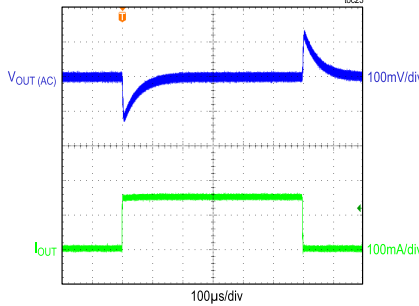
CONDITIONS: 5V OUTPUT, PWM MODE
