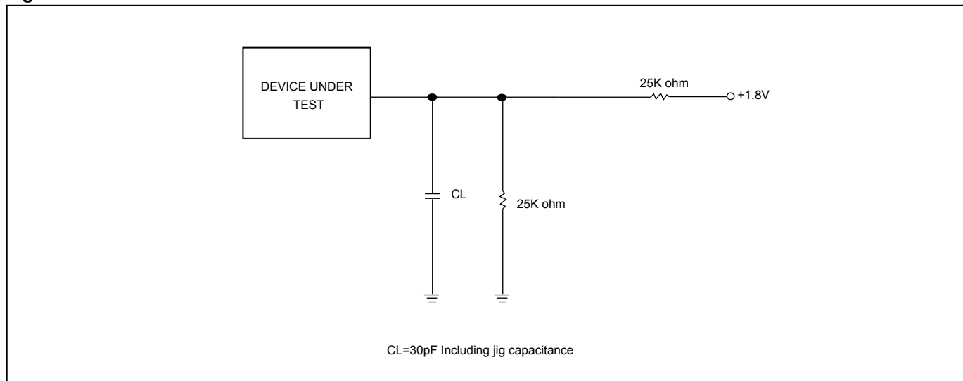
Figure 105. OUTPUT LOADING
