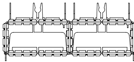
FIG 6 QSFP-1-2-S-LP-F SHOWN (DIFFERENT AS SHOWN, OTHERWISE SAME AS FIG 3 & 4)
