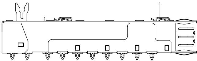
FIG 6 QSFP-1-2-S-LP-F SHOWN (DIFFERENT AS SHOWN, OTHERWISE SAME AS FIG 3 & 4)
