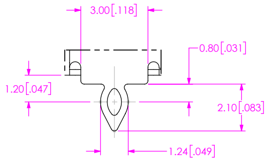
DETAIL 'H' SCALE 6 : 1
