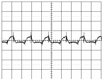
Output voltage ripple (20mV/div.) at: T_{ref} = +25^{\circ}\text{C} , I_O = 6\text{ A} resistive load, V_i = 3.3\text{ V} . Time scale: 1 \mu\text{s} /div. See the filter in the Output ripple and noise section (EMC Specification).
