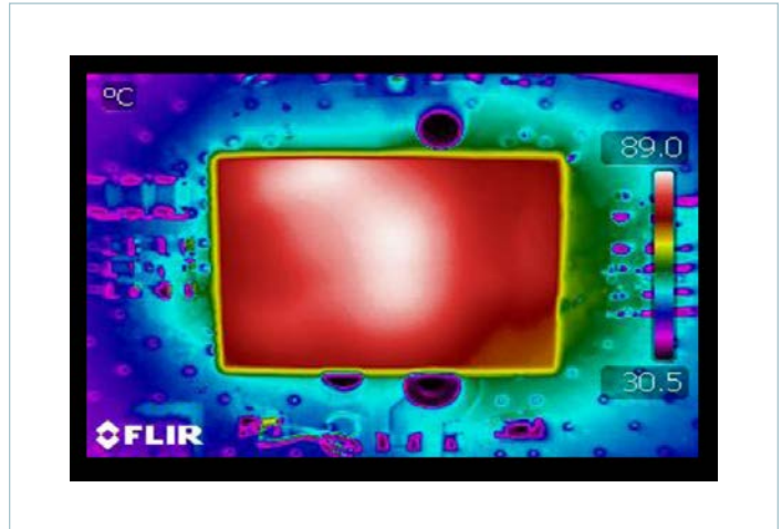
Figure 20 — Thermal image ( V_{IN} = 48V , I_{OUT} = 5A , CR, OLFM evaluation PCB)
