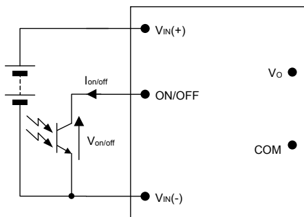
Figure 40. Circuit configuration for using Remote On/Off Implementation.
