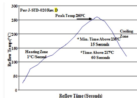
Figure 51. Recommended linear reflow profile using Sn/Ag/Cu solder.
