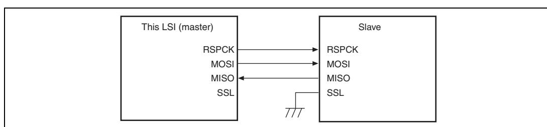
Figure 16.2 Master/Slave Configuration Example (This LSI = Master)
