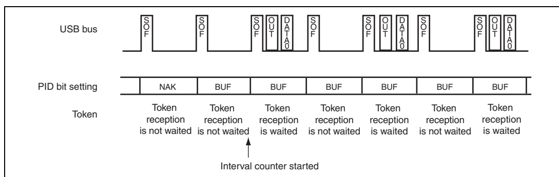
Figure 26.19 Relationship between (μ) Frames and Expected Token Reception when IITV = 1
