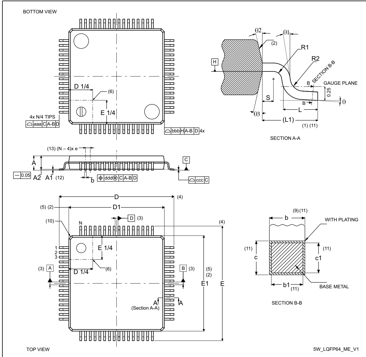
Figure 44. LQFP64 - Outline (15)
