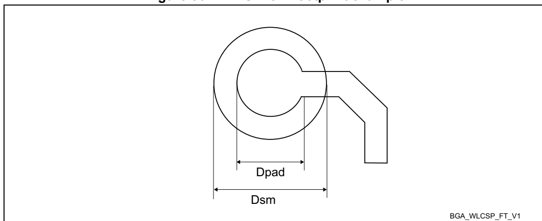
Figure 36. WLCSP25 - Footprint example
