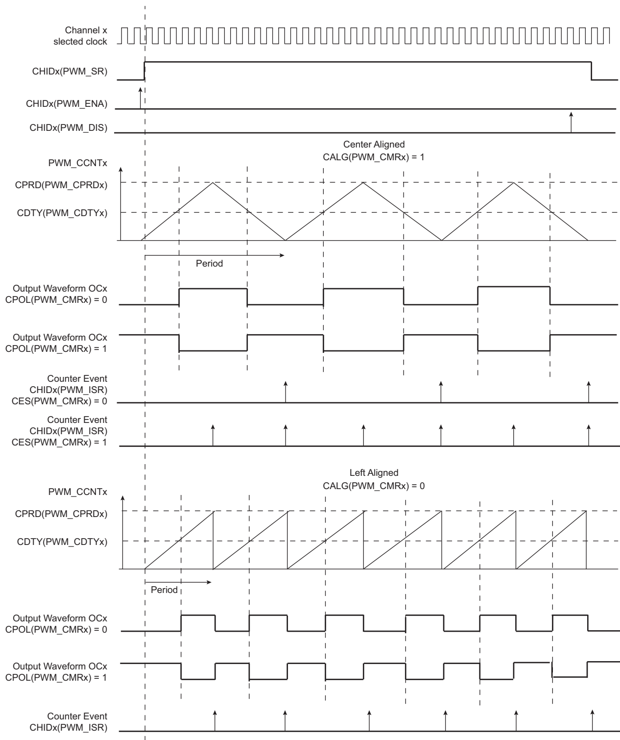
Figure 39-5. Waveform Properties
