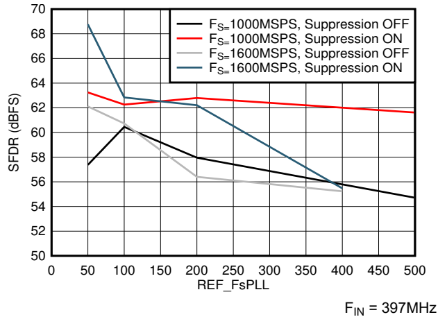
Figure 8-39. SFDR vs F_{REF} and Suppression
