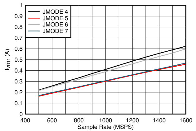
Figure 8-84. Quad Channel, I_{VDD11} vs F_S
