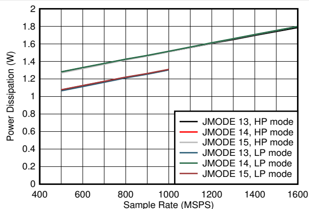
Figure 8-92. Dual Channel, Power Dissipation vs F_S and JMODE 13 - 15
