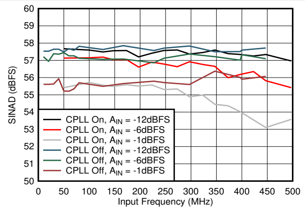
Figure 8-56. SINAD vs A_{IN} and C-PLL
