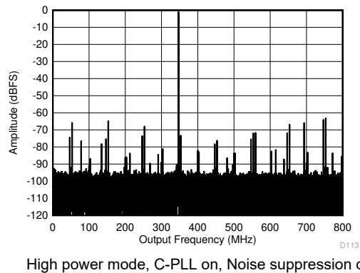
Figure 8-6. Single Tone FFT at 347 MHz and -1 dBFS
