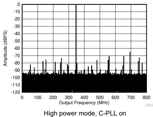
Figure 8-5. Single Tone FFT at 347 MHz and -1 dBFS
