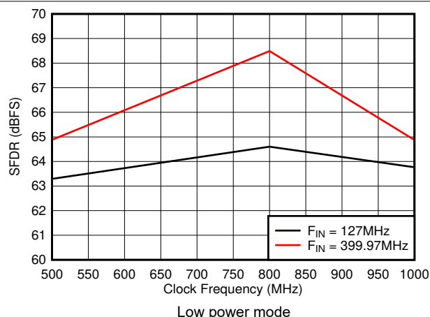
Figure 8-27. SFDR vs Sample Rate
