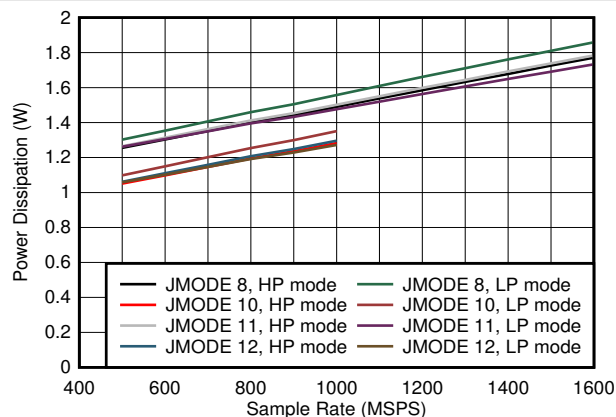
Figure 8-91. Dual Channel, Power Dissipation vs F_S and JMODE 8 - 12
