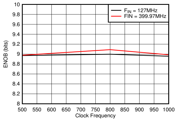
Figure 8-31. ENOB vs Sample Rate
