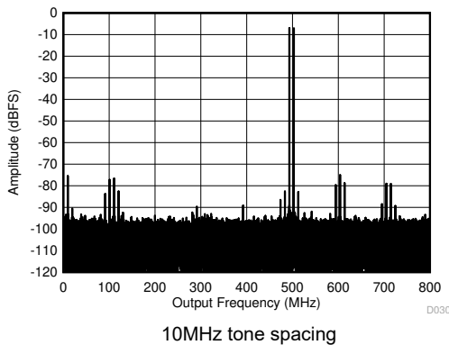
Figure 8-69. Two Tone FFT at 498MHz
