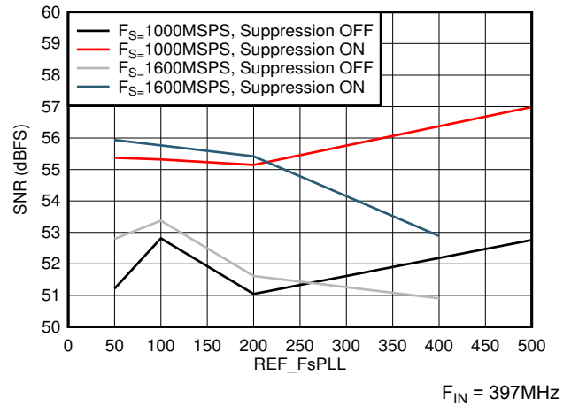
Figure 8-38. SNR vs F_{REF} and Suppression
