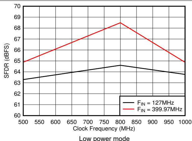
Figure 8-29. SFDR vs Sample Rate
