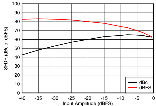
Figure 8-32. SFDR vs A_{IN}
