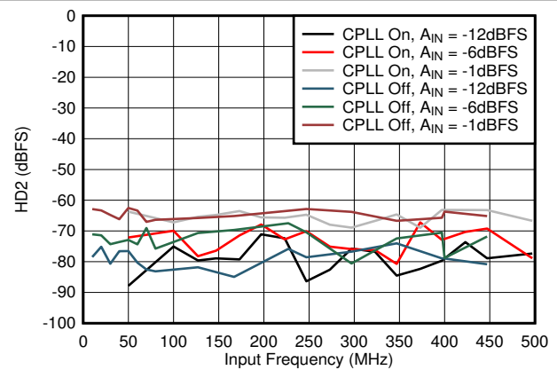
Figure 8-58. HD2 vs A_{IN} and C-PLL
