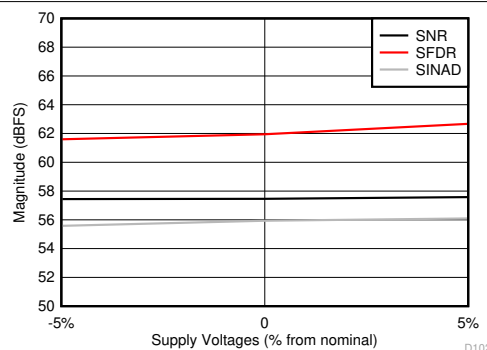
Figure 8-62. SNR, SFDR and SINAD vs Supply Voltages
