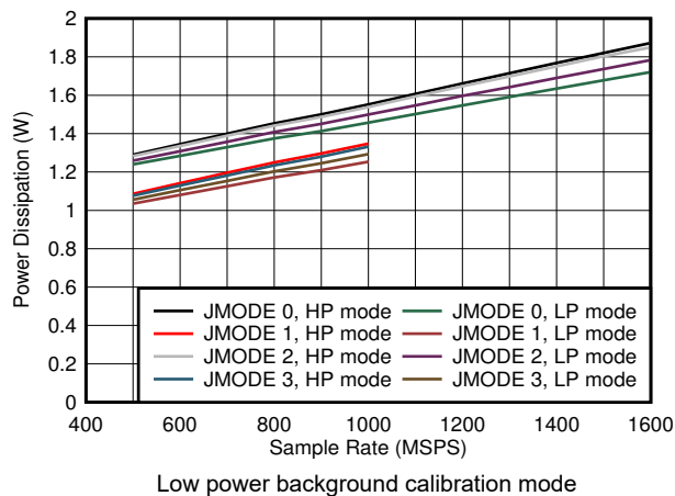
Figure 8-89. Dual Channel, Power Dissipation vs F_S and JMODE 0 - 3
