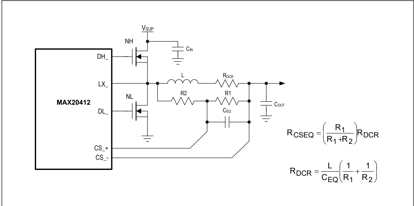
Figure 8. Current-Sense Configurations
