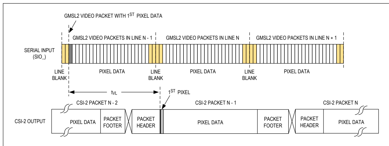
Figure 9. GMSL2 Video Latency
